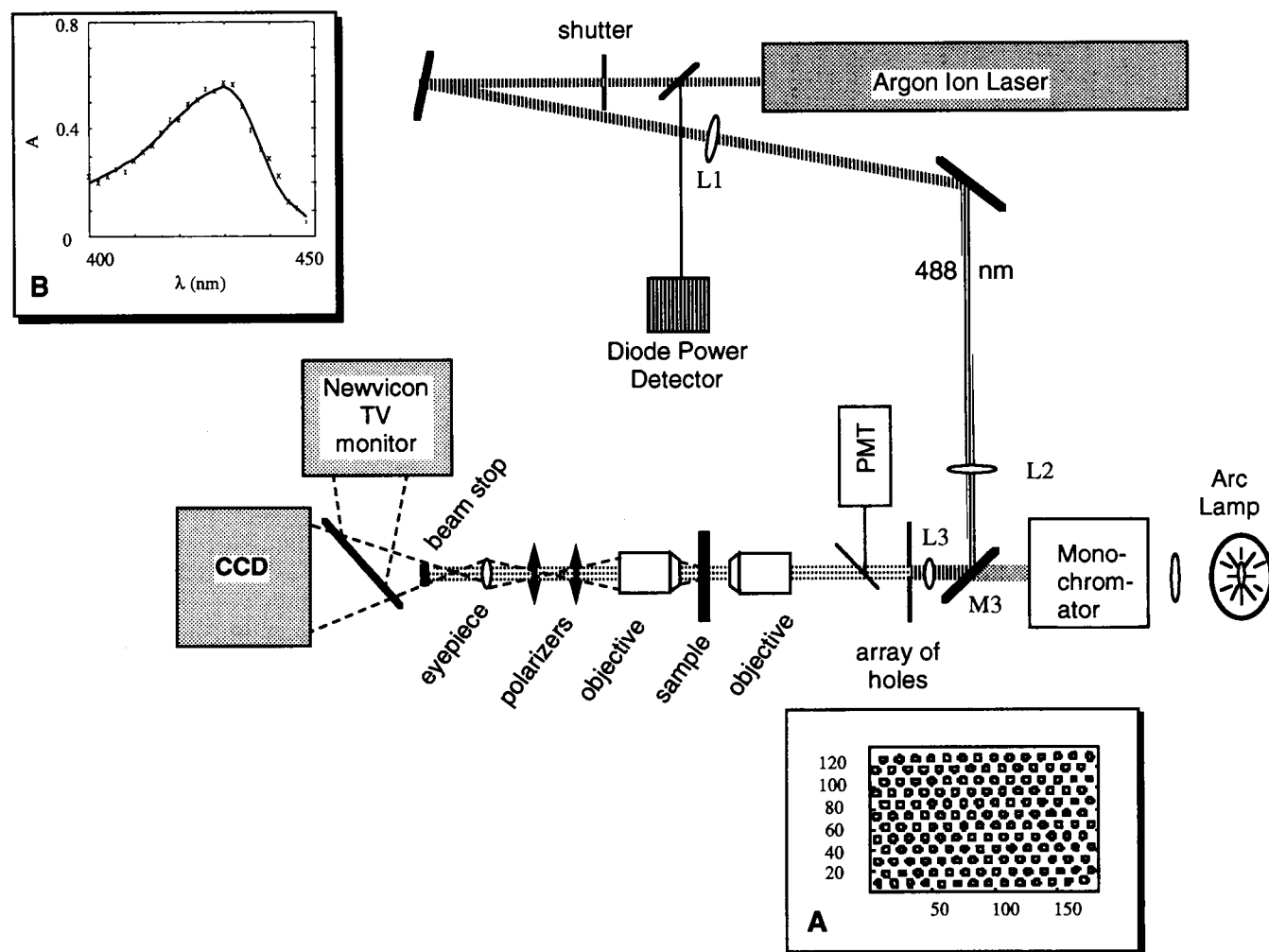
FIGURE 1 A schematic of the apparatus. The sample is observed by a 10 \times Leitz LWD strain-free objective, and its image is projected onto a CCD camera and a TV monitor. For light scattering measurements, the beam of an argon ion laser is sent through an array of holes placed where a field diaphragm is conventionally located. These holes are imaged at the sample. To reject the direct laser light, polarizers are placed after the collecting objective. In addition, a beam stop is placed at a position after the eyepiece, which is conjugate to the back aperture of the collecting objective. Thus light scattered at a greater angle than that of the laser passes the stop and is imaged at the CCD. M3 is a partially reflecting mirror that passes light in the Soret band region (400–450 nm) while reflecting the laser line at 488 nm. For absorbance measurements the beam stop may be removed. In some absorbance measurements, a pair of filters is also placed before the CCD. For absorbance, the light is provided by a 150-W xenon lamp and passed through a monochromator. The reference photomultiplier (PMT) is used for measurement of absorbance spectra. A MacII fx computer controls the CCD data transfer, as well as the shutter for the laser, and the stepping of the monochromator. ( Inset A ) Image of the array of holes taken with the CCD camera. ( Inset B ) Absorbance spectrum taken with the laser on. Note that the sample has been converted to deoxyHb, and that an absorbance spectrum of good quality can be recorded, despite a laser beam with intensity that is orders of magnitude greater.
