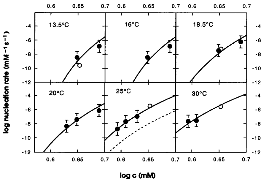
FIGURE 5 Nucleation rates f_0 as a function of concentration for different temperatures as shown. Rates are obtained by fitting distributions similar to those shown in Fig. 4. The solid lines are the best fit obtained by varying a single parameter, the chemical potential of the monomer contacts, \mu_{PC} . The chemical potentials so obtained are shown in Fig. 6. A single data point collected at 35°C is not shown. The open circles are the results obtained by Hofrichter (1986), using a serial technique, and have not been included in determining the best-fit line. The data of Hofrichter were taken at 14.3°C, 18.9°C, and 29.2°C, and the point at 25°C was interpolated in the original paper. It is a mark of the success of the nucleation theory employed that fits to one set of data extrapolate correctly to the other data set. The error bars in the data are primarily due to variations of the volume V in Eq. 2 due to variation of thickness across the sample and variation in imaged spot size.
